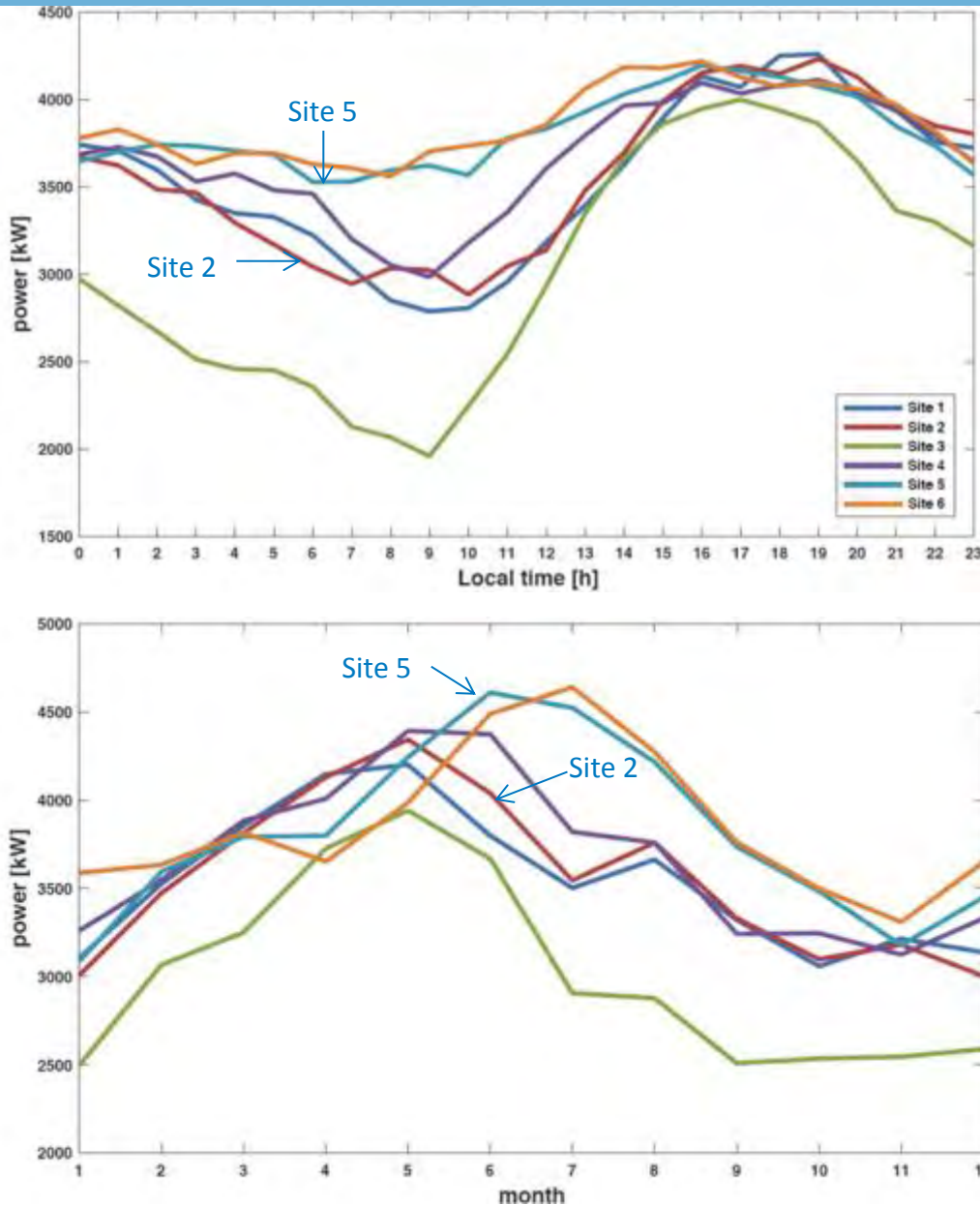
Figures: Diurnal and monthly single 6 MW turbine output for six California floating wind reference sites (top left Diurnal) and (Bottom left – monthly average)
