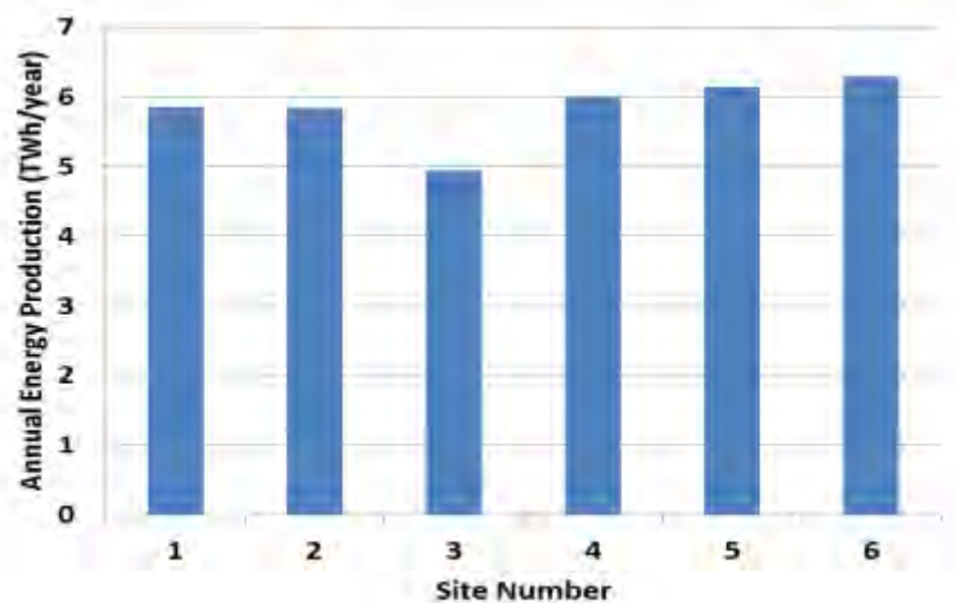
Annual Energy Production (AEP) by site with 1200 MW deployed on each site
