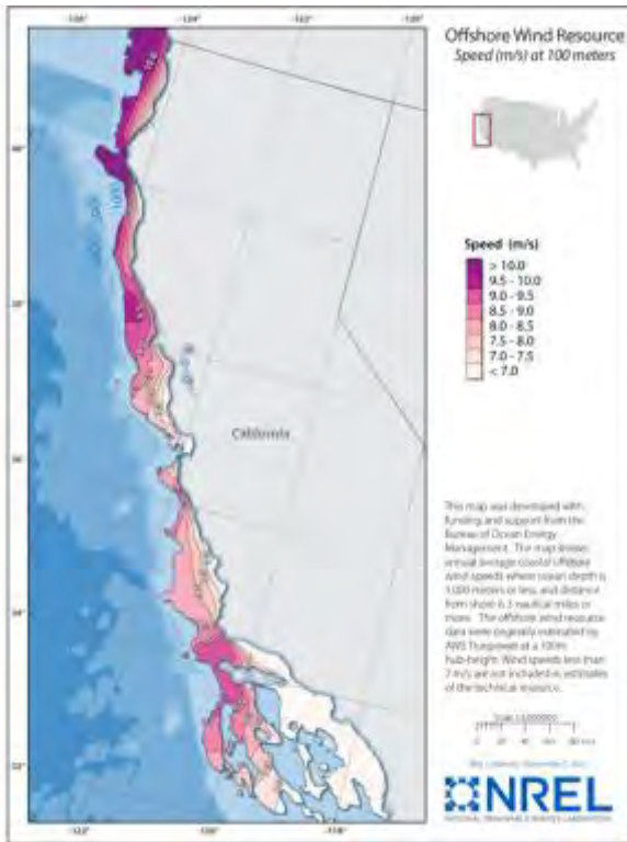
Technical offshore wind resource
