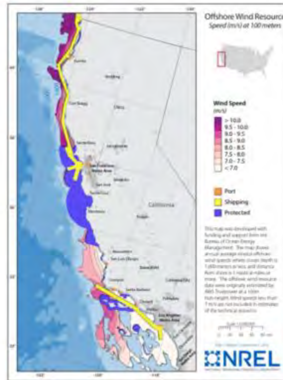
Technical offshore wind resource and Black and Veatch exclusion data layer
