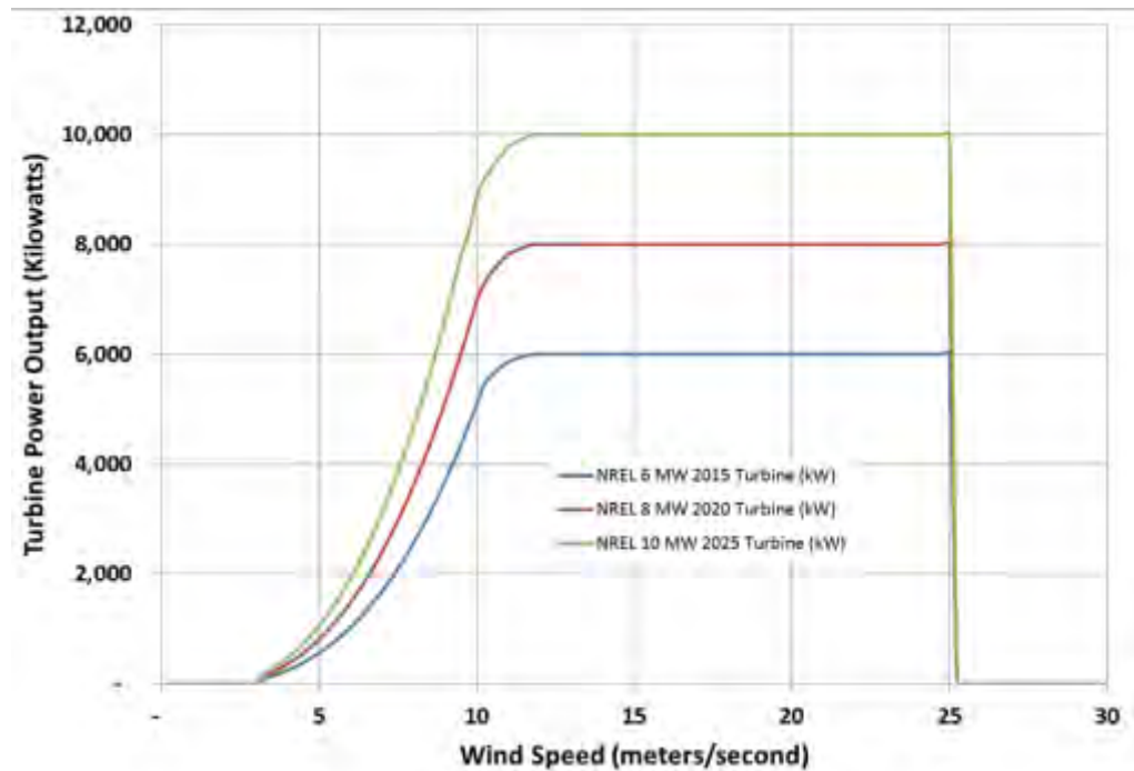
Generic power curves used to calculate Annual Energy Production (AEP)
